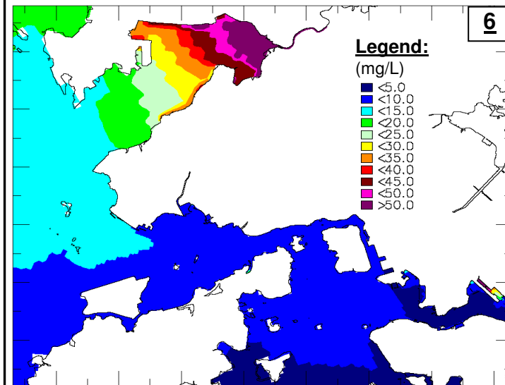
Scenario 4b (Emergency Discharge at Bypass Location)
