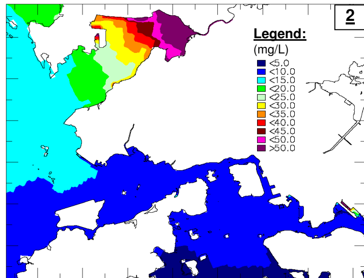
Scenario 3b (Emergency Discharge at Bypass Location)
