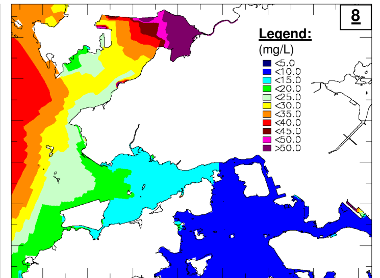
Scenario 4b (Emergency Discharge at Bypass Location)
